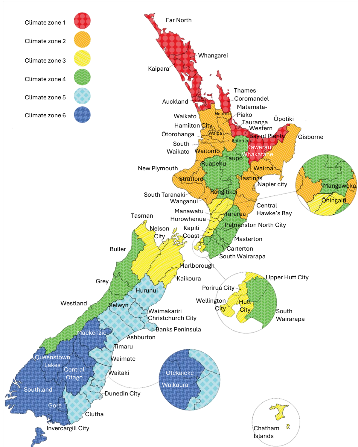
Figure C.1.1.2: Map of New Zealand climate zones
