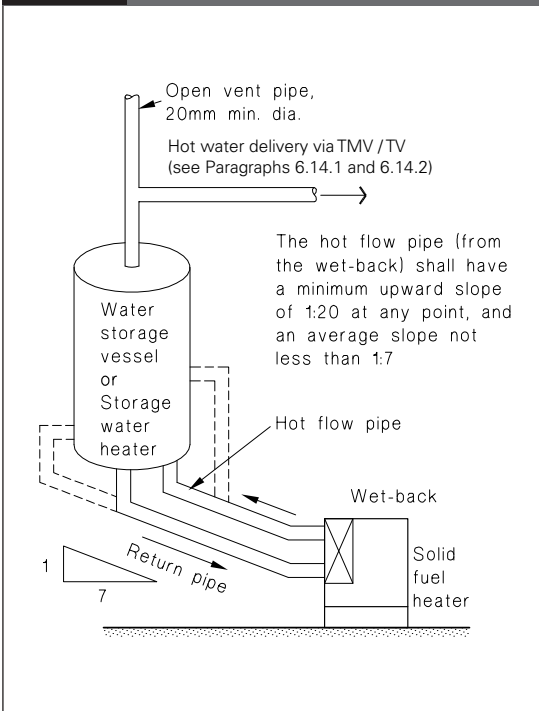
Figure 15: Wet-back Installation – Open Vented System Paragraph 6.13.1 b)
