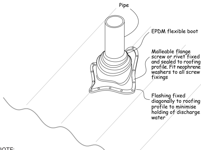
Figure 6: Flashing for pipes, cables and other penetrations Paragraphs 5.2.4 and 5.2.5 a)
