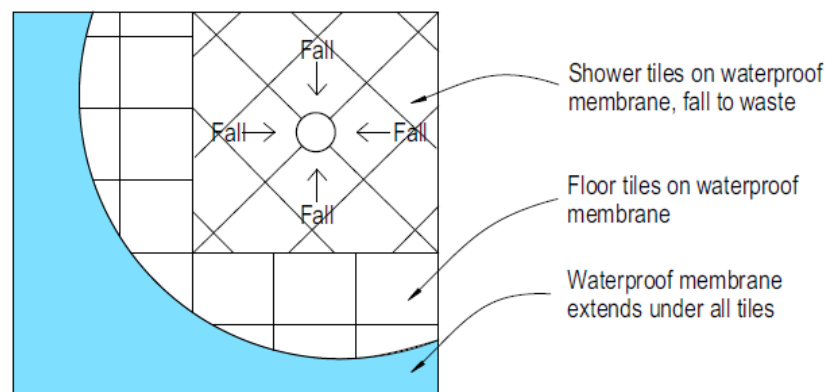
Figure 35: Recommended layout for tiles in shower areas with centre waste
