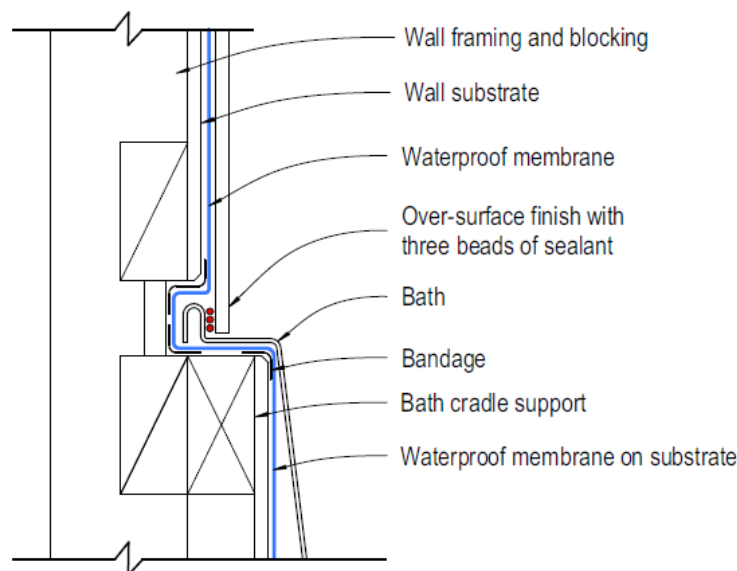
Figure 31: Bath sealed to wall, membrane behind over-surface finish
