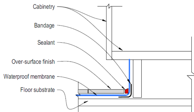
Figure 17: Waterproof membrane system installed after cabinetry
