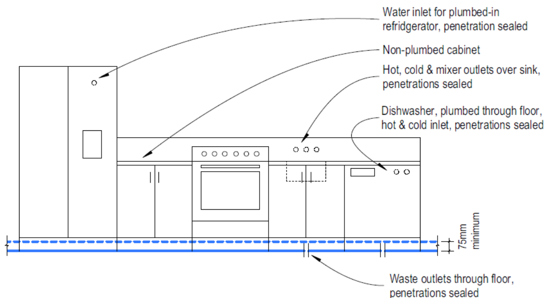
Figure 5: Extent of waterproof membrane behind kitchen cabinets
