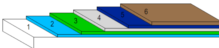
Figure 40: Sound insulation layer only, if installed on an existing slab
