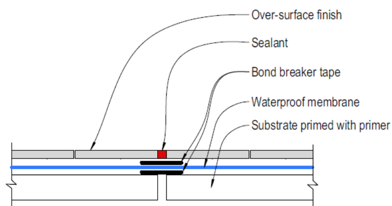
Figure 23: Waterproof membrane system over a control joint in the substrate
