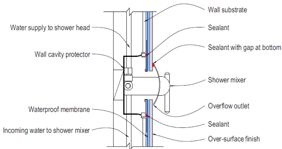
Figure 29: Waterproof membrane system around wall penetration in shower area with over-surface finish
