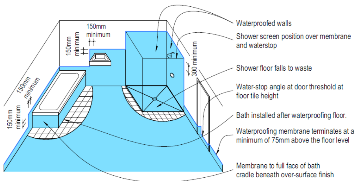
Figure 6: Extent of membrane in bathroom with hobless shower area
