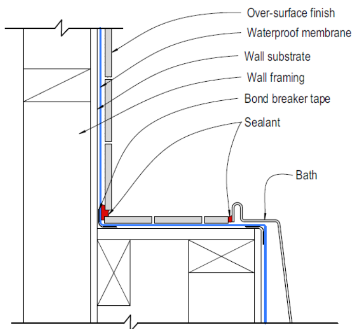
Figure 34: Bath with tiled surround
