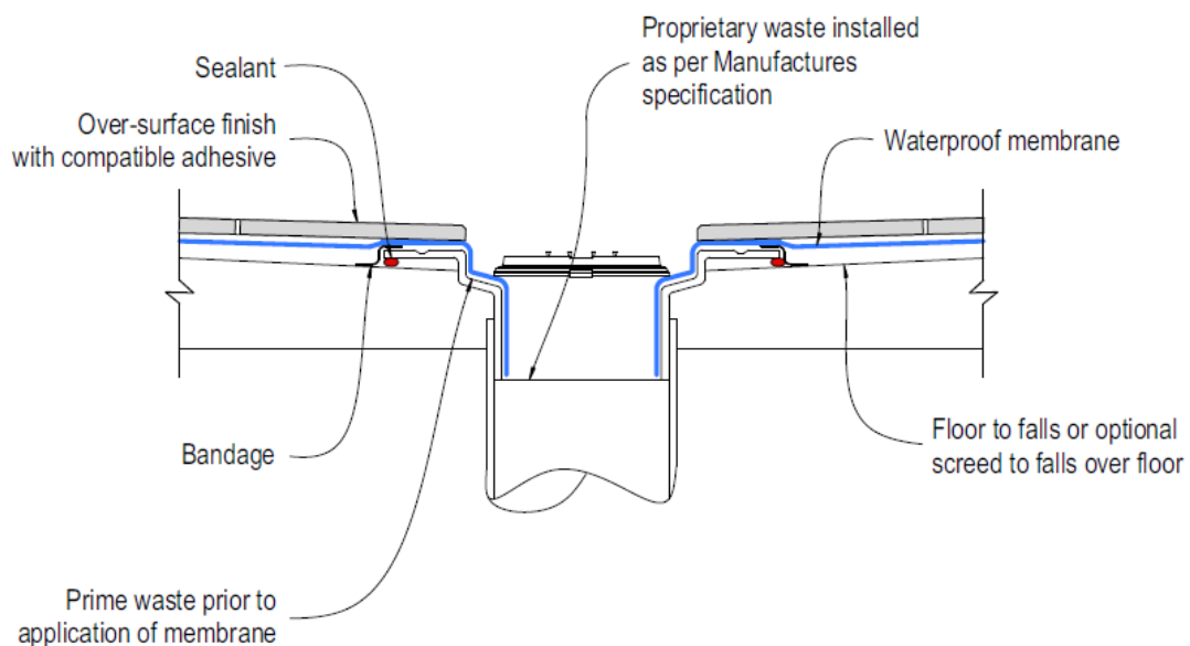
Figure 27: Waterproof membrane system into floor waste outlet
