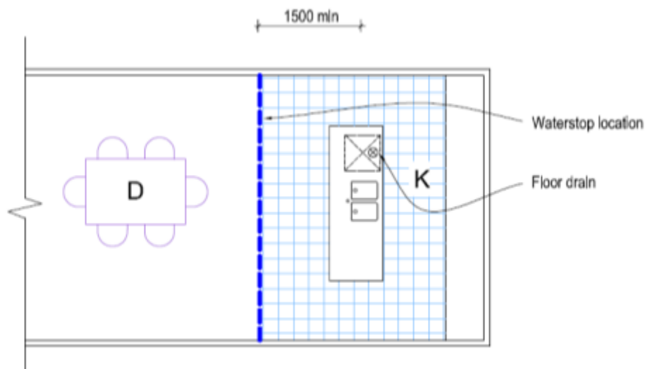
Figure 3: Extent of waterproof membrane system for an island bench with sink in the island
