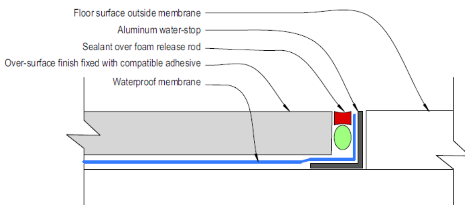
Figure 14: Water-stop at termination of waterproof membrane system
