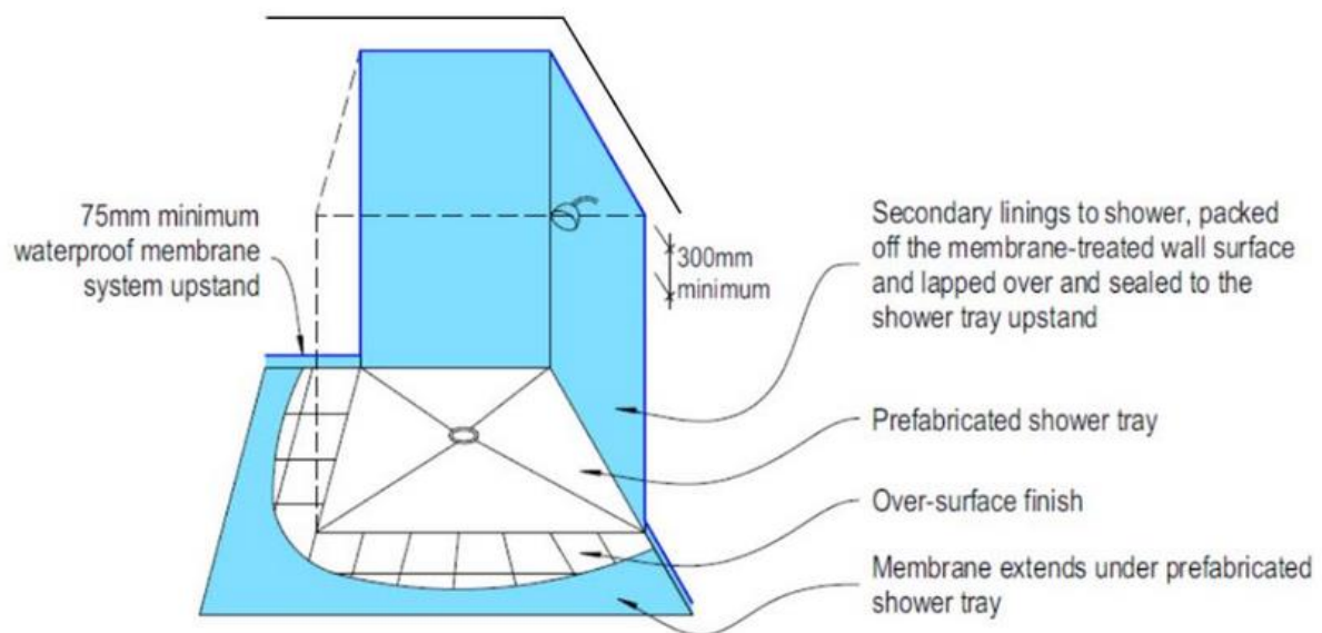
Figure 12: Extent of waterproof membrane system for shower areas
