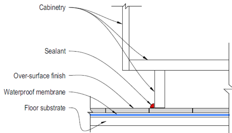
Figure 16: Tiles and waterproof membrane system under cabinet
