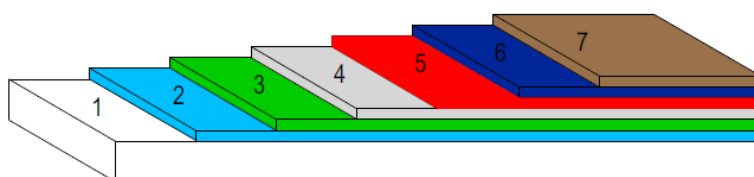
Figure 42: Heating and sound insulation layers, if installed on an existing slab
