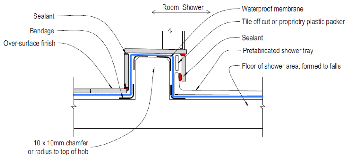
Figure 26: Typical shower area with prefabricated shower tray
