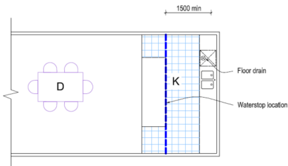
Figure 2: Extent of waterproof membrane system for island bench with sink at the back bench
