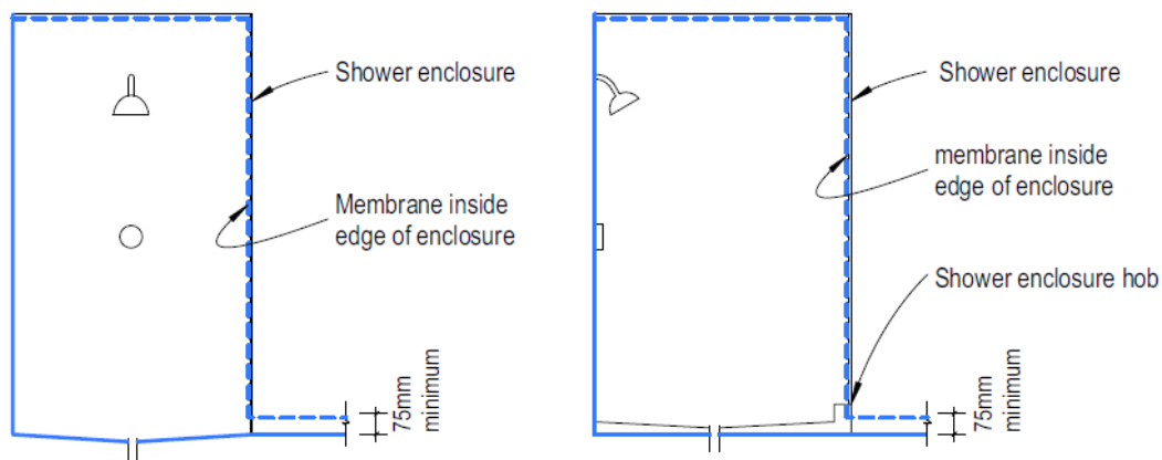
Figure 8: Extent of waterproof membrane behind shower enclosures
