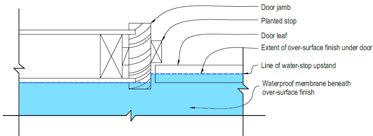
Figure 18: Plan view of water-stop under door jamb
