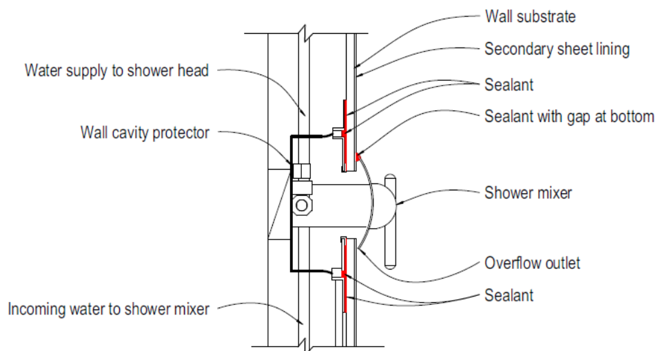
Figure 30: Waterproof sealing around wall penetration in shower area with a secondary sheet lining
