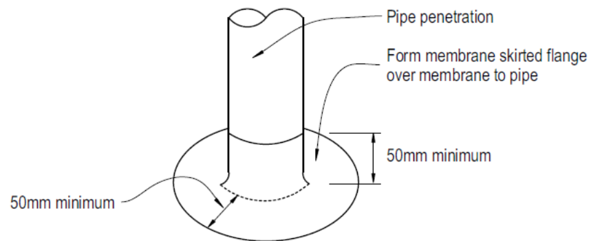
Figure 28: Pipe penetrations
