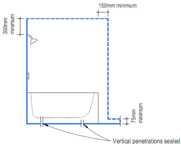
Figure 9: Extent of waterproof membrane of shower over bath
