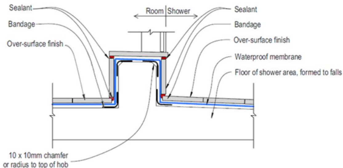
Figure 25: Typical formed shower area with integral hob
