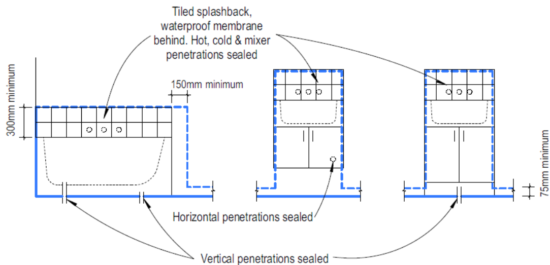
Figure 7: Extent of waterproof membrane behind bathroom fittings
