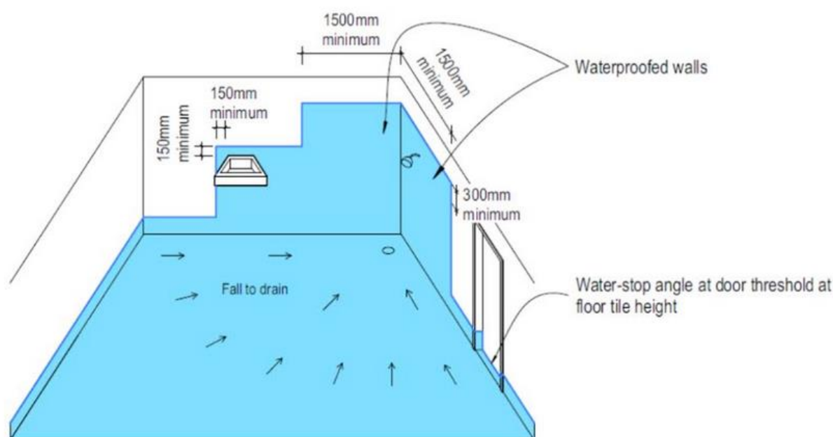
Figure 11: Typical layout of bathroom for an open shower area
