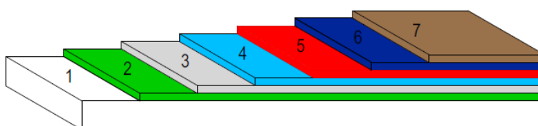
Figure 41: Heating and sound insulation layers, if installed on a new slab
