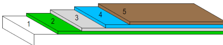
Figure 39: Sound insulation layer only, if installed on a new slab
