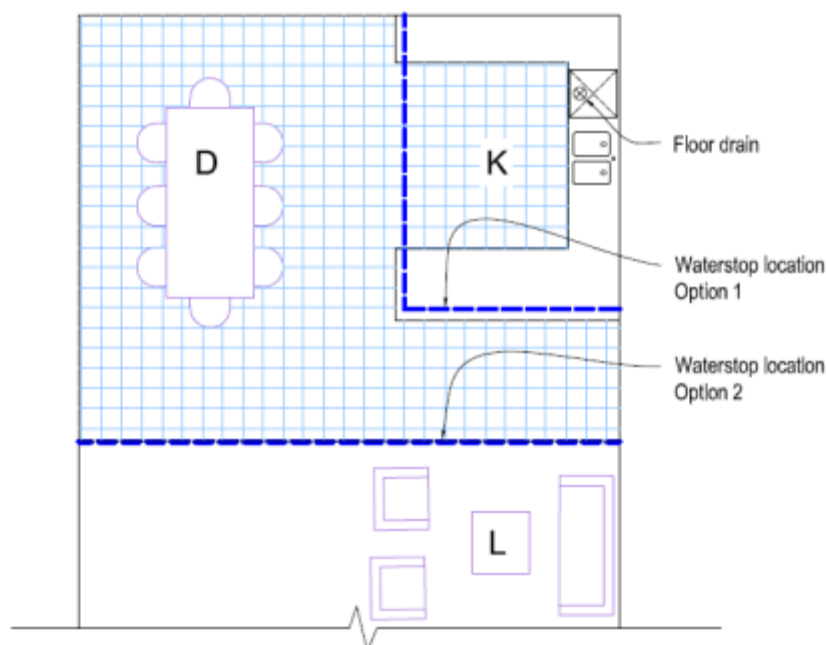
Figure 4: Extent of waterproof membrane system for an open-plan kitchen/dining/living room
