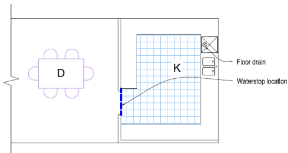
Figure 1: Extent of waterproof membrane system for separate kitchen
