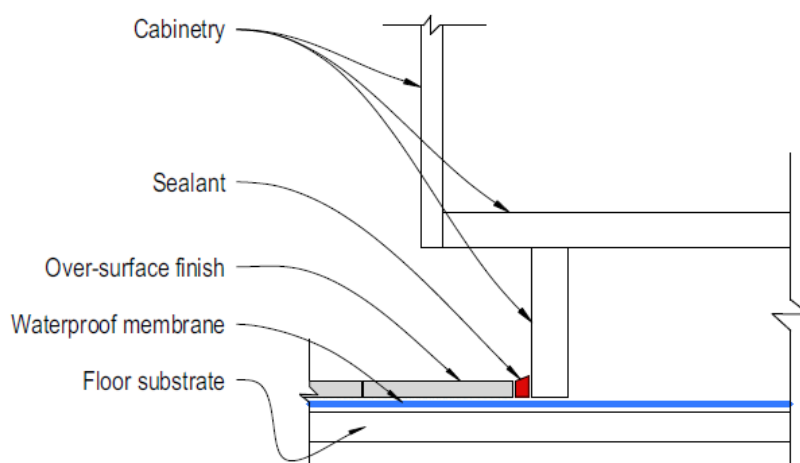
Figure 15: Waterproof membrane system installed before cabinetry
