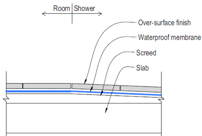
Figure 24: Typical tiled shower area with no hob
