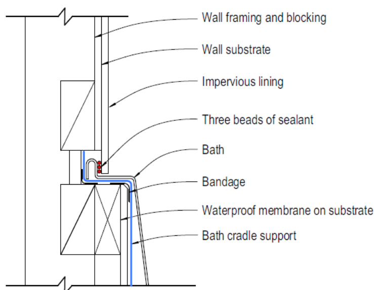
Figure 32: Bath sealed to wall, no membrane behind impervious lining
