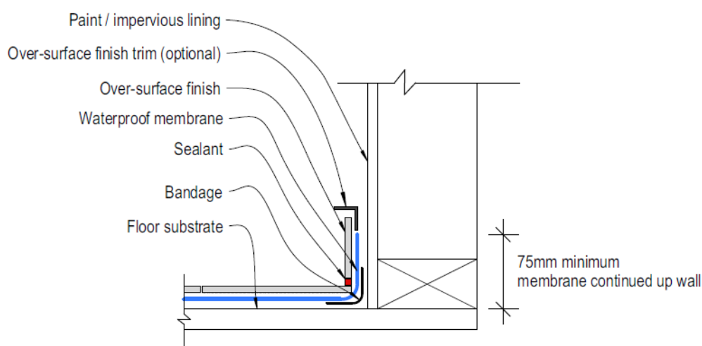
Figure 21: Waterproof membrane system behind skirting
