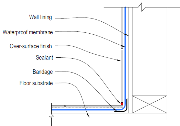
Figure 22: Waterproof membrane system behind over-surface finish to walls
