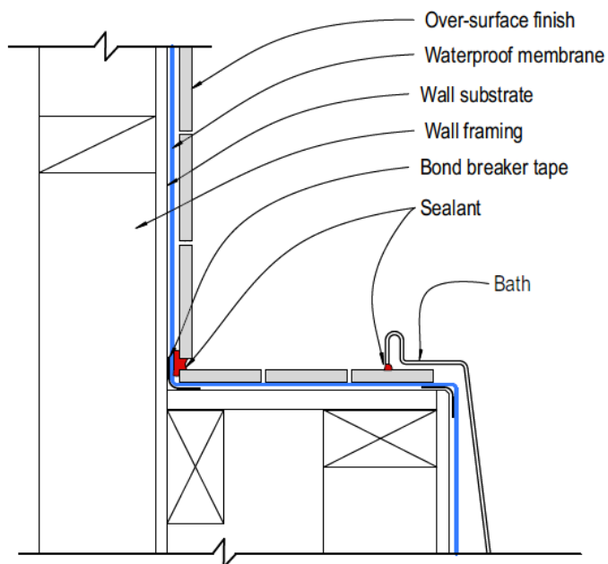
Figure 33: Bath over tiled surround
